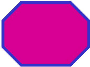
Octagon
