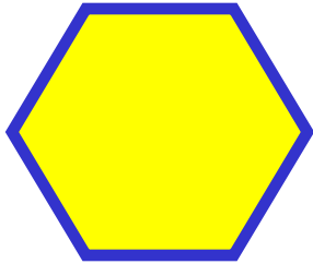
Hexagon
